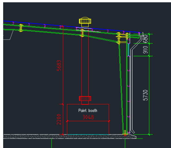
Sketch of a paint booth with a vent duct
